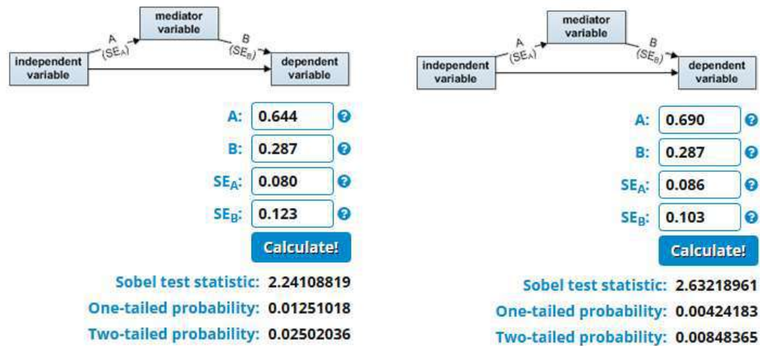
Fig. 5. Sobel Test Statistic (APWB → EDC → OA and APWB → EA → OA)
